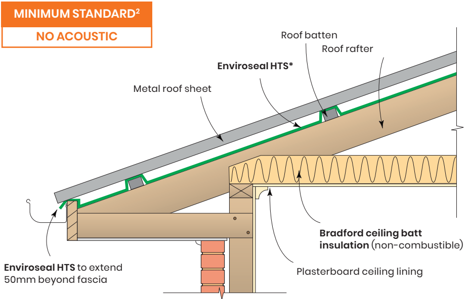
Figure 4.2.1.b Fascia Detail – Metal Roof (BAL12.5 – 40)
