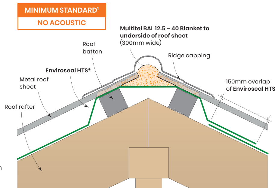
Figure 4.2.4.c Hip/Ridge Detail – Steel Roof (BAL-12.5 – BAL-40)
