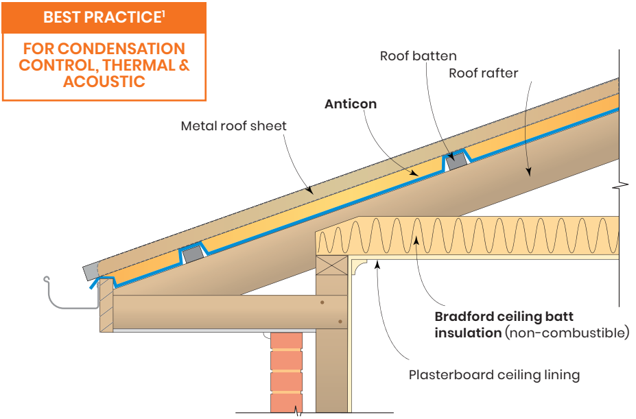
Figure 4.2.1.a Fascia Detail – Metal Roof (BAL12.5 – 40)
