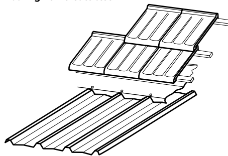
Flashing from tiles to steel
