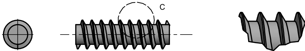
Buttress Thread
